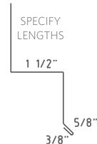
Counter Flashing CF1
