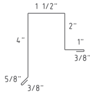
Gable G4
