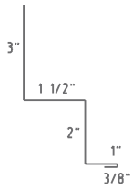
Sidewall S4
