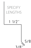
Counter Flashing CF1
