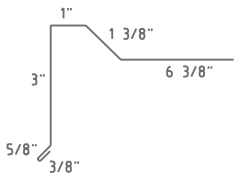
Chalet Gable CG1
